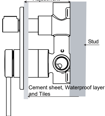
Mixer with diverter: 45mm to 70mm Adjustment
