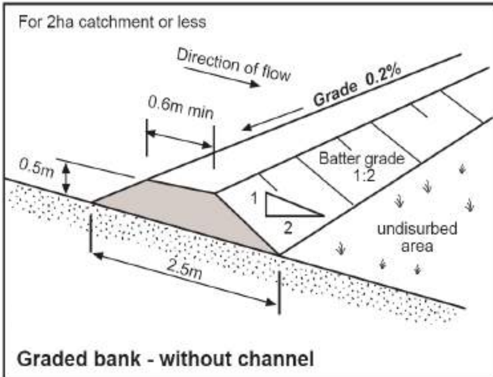
Figure 1 - Graded Banks
