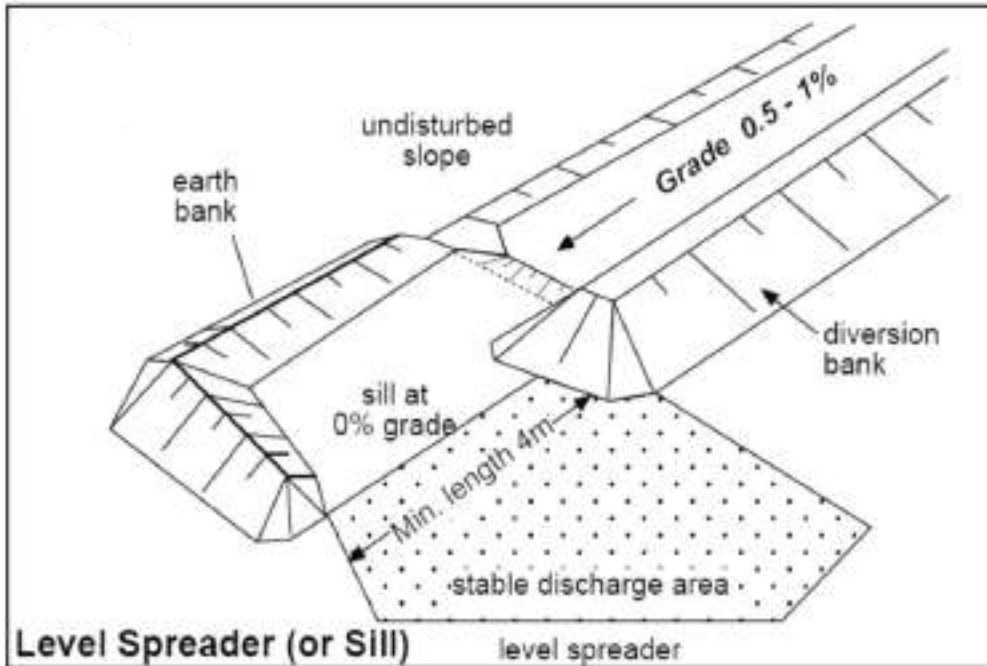
Figure 3 - Level Spreader
