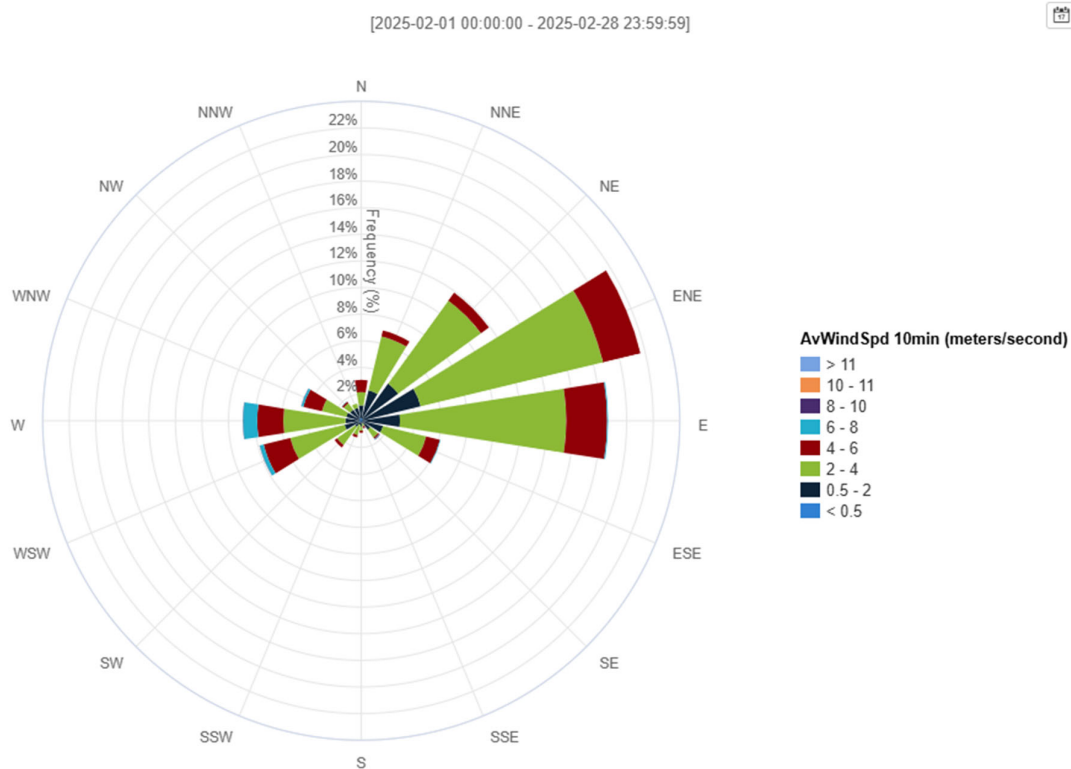
Figure 3-1 Wind rose for February 2025
