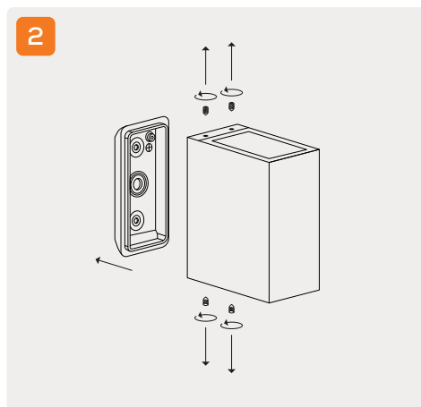
Remove back plate.
