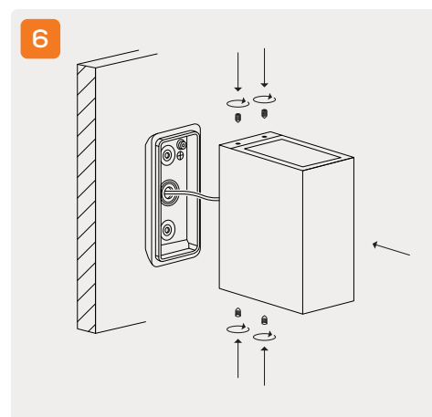
Attach fitting to mounted back plate.
