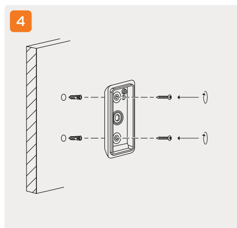
Mount back plate to wall.
