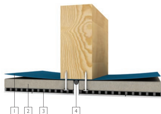
Figure 15 Relief joint details
