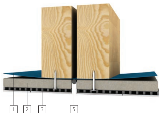
Figure 14 Control joints details
