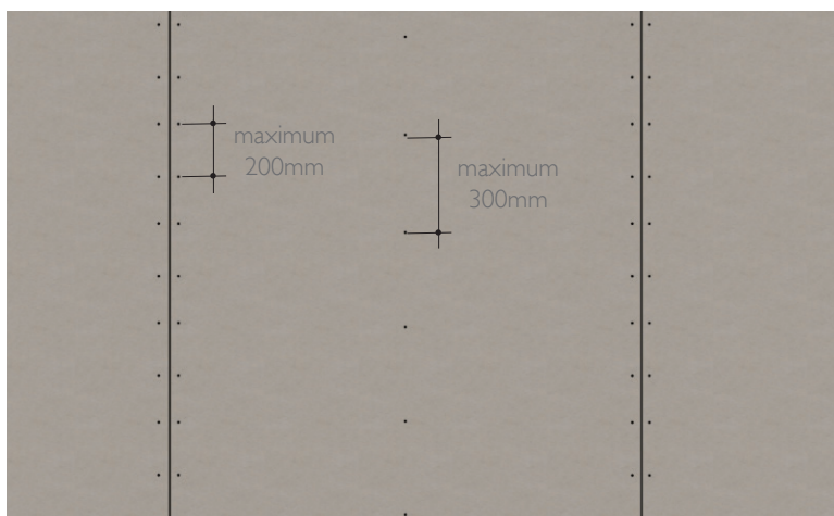
Figure 11 Fastening position
