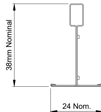
TRUGRID T24 SCALE Full Size
