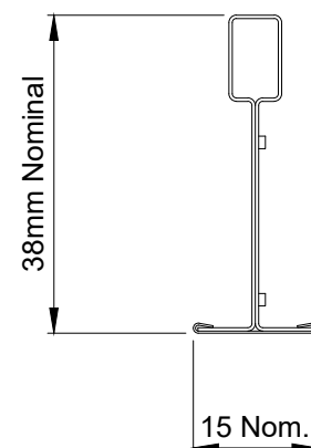
TRUGRID T 15 SCALE Full Size
