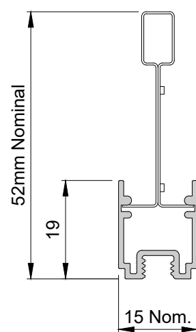
ALUGRID Q 15/19 SCALE Full Size
