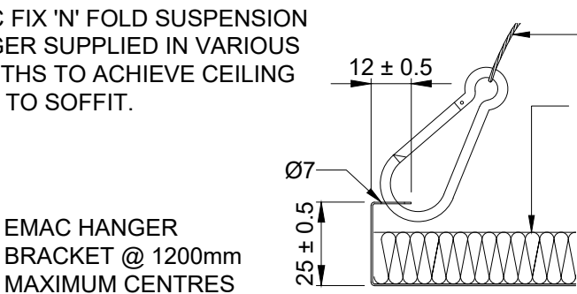
DETAIL 1 (OPTIONAL SAFETY CABLE) SCALE 1:2
