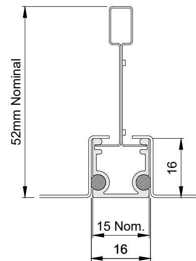
Alugrid - P 15/16 (CLEANSEAL)
