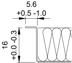
DETAIL 3 (OUT-TURN FLANGE) SCALE Full Size
