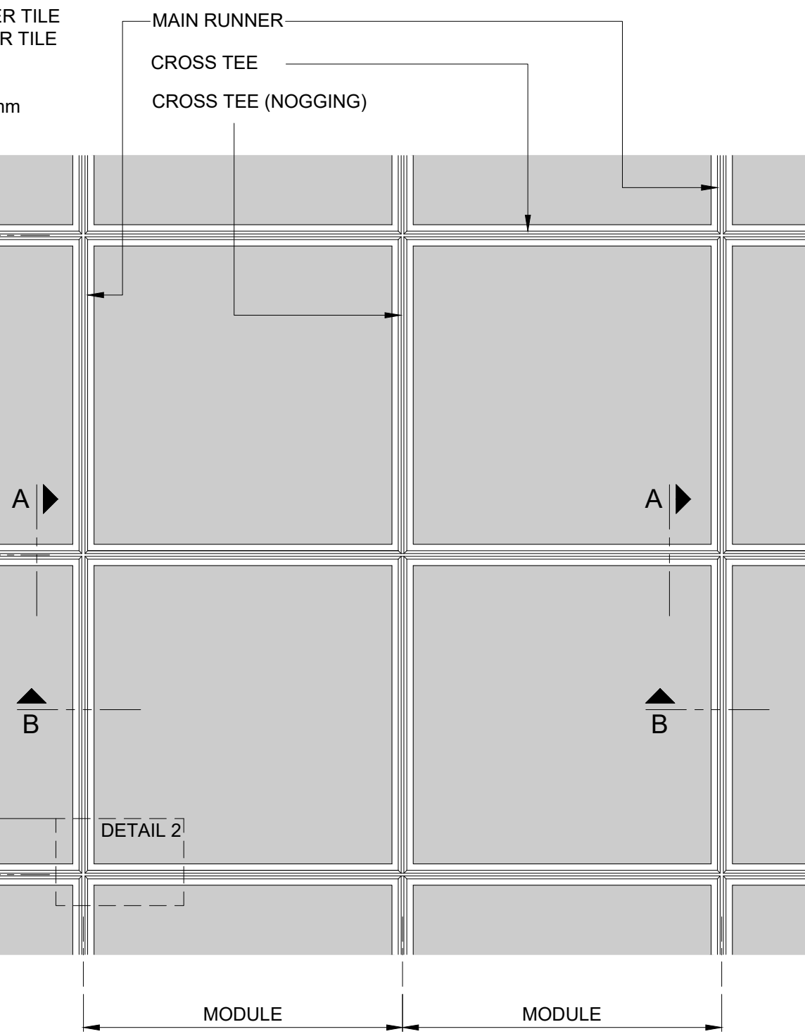
PART REFLECTED CEILING PLAN SCALE 1:10
