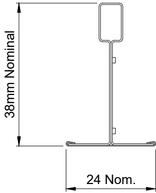
TRUGRID T24 SCALE Full Size
