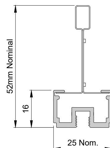
ALUGRID Q 25/16 SCALE Full Size
