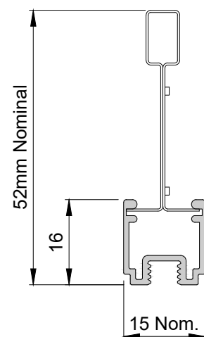
ALUGRID Q 15/16 SCALE Full Size
