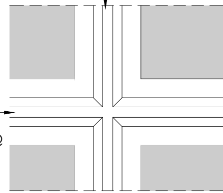
DETAIL 1 (MAIN RUNNER & CROSS TEE JUNCTION) SCALE 1:2
