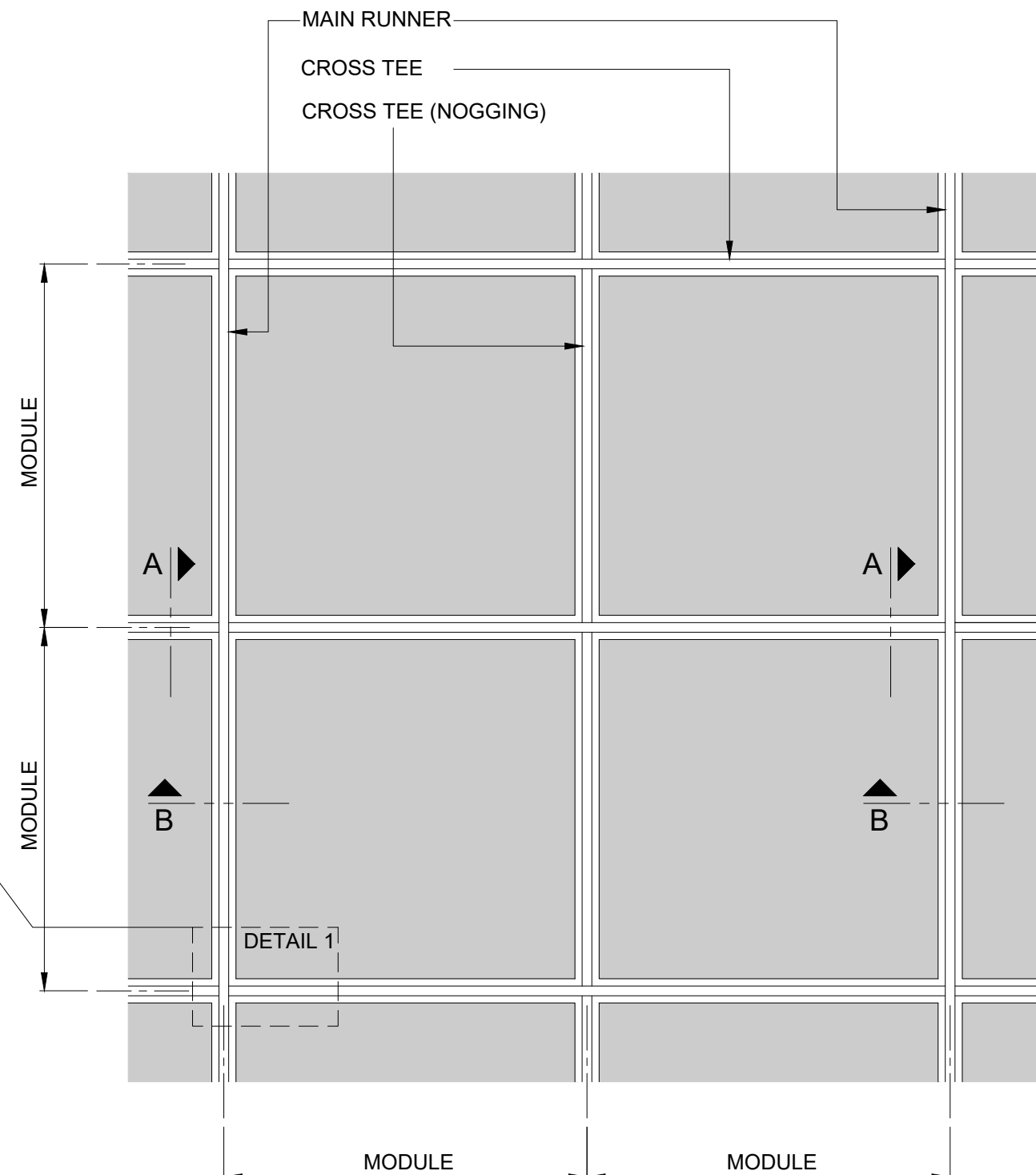
PART REFLECTED CEILING PLAN SCALE 1:10
