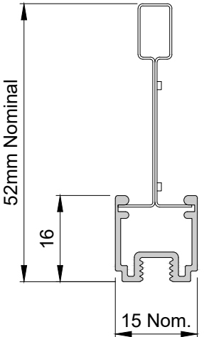
ALUGRID Q 15/16 SCALE Full Size
