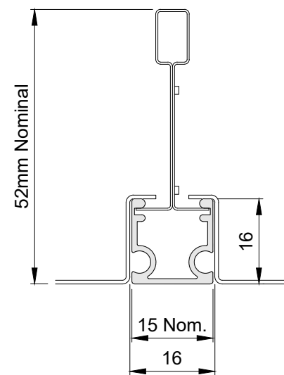
Alugrid - P 15/16 PLAIN
