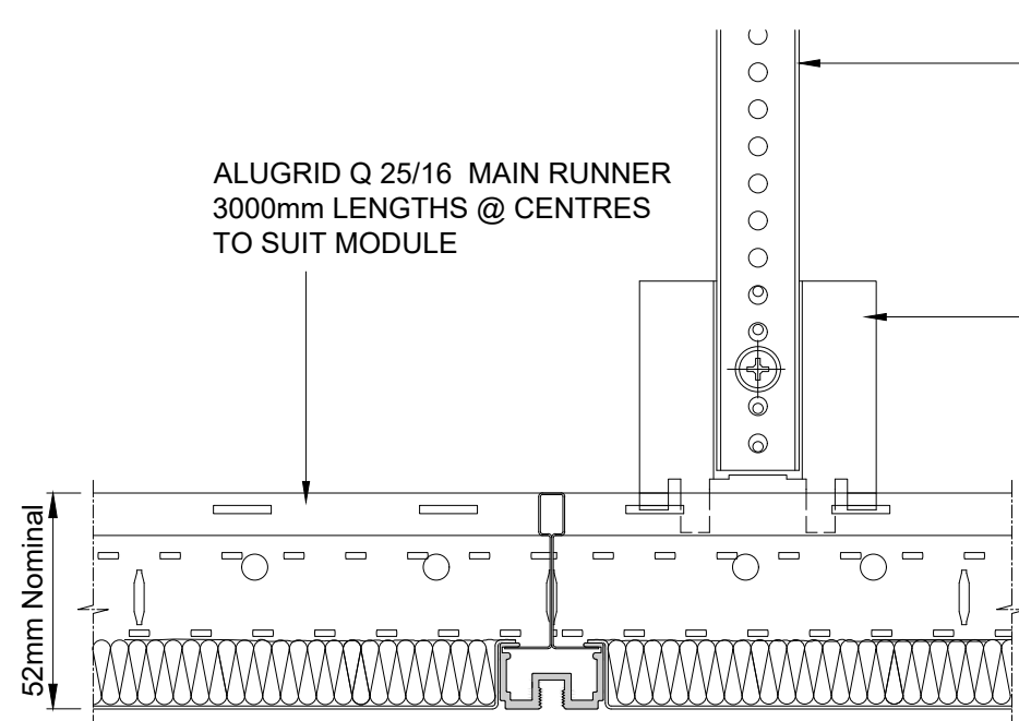
SECTION 'A' SCALE 1:2
