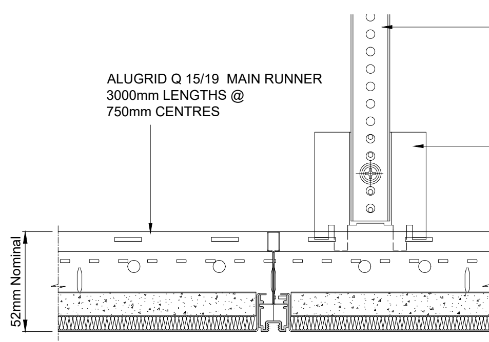
SECTION 'A' SCALE 1:2
