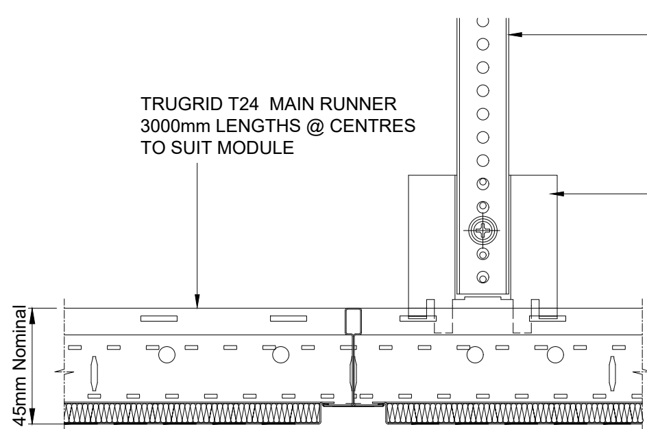
SECTION 'A' SCALE 1:2
