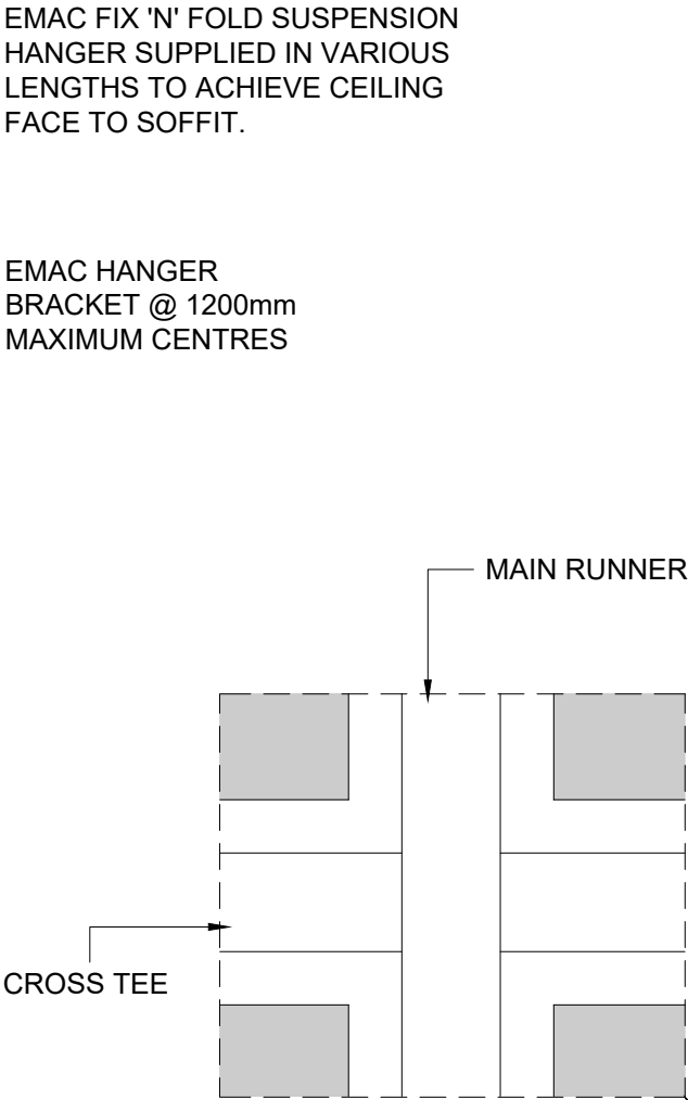
DETAIL 1 (MAIN RUNNER & CROSS TEE JUNCTION) SCALE 1:2
