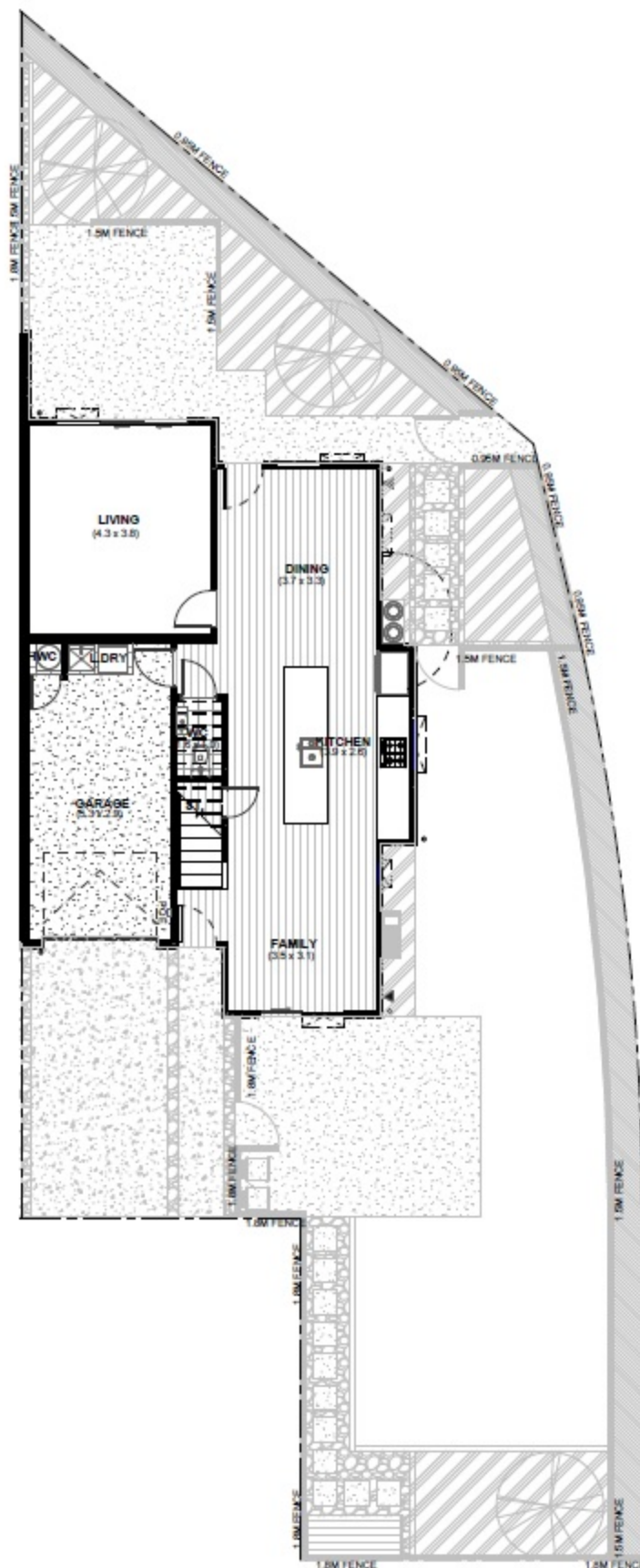
LOT 624 - GROUND FLOOR PLAN
