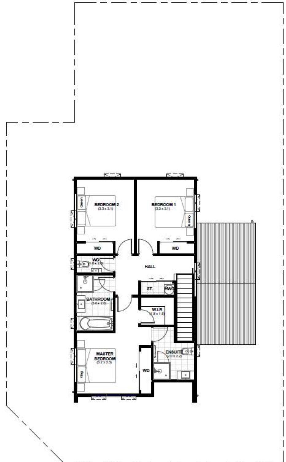
LOT 182 - FIRST FLOOR PLAN
