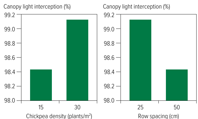
Figure 19: The effect of chickpea density (plants/m 2 ) (left) and row spacing (cm) (right) on canopy light interception (%).
