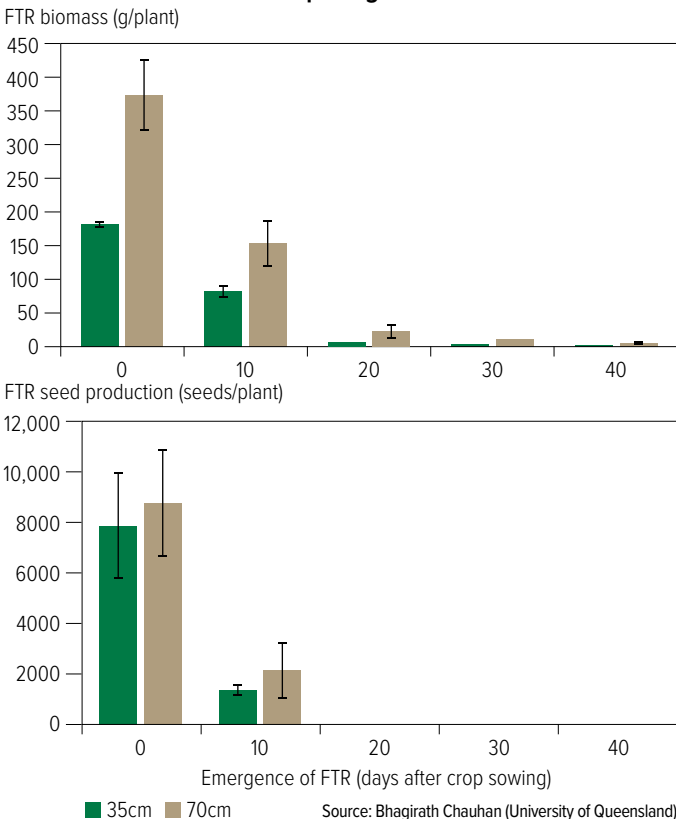
Figure 13: Delayed emergence of FTR in a mungbean crop reduced FTR growth and seed production. This effect was enhanced at a narrow row spacing of 35cm.
