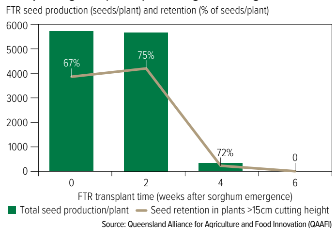
Figure 14: FTR seed production (seeds/plant) and retention (% of seeds/plant) in sorghum in response to different transplanting time (weeks) after sorghum emergence
