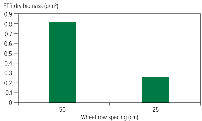
Figure 18: The effect of wheat row spacing (cm) on the growth of FTR transplanted late into wheat. The FTR were assessed near crop harvest and had not produced any seed by this time.
