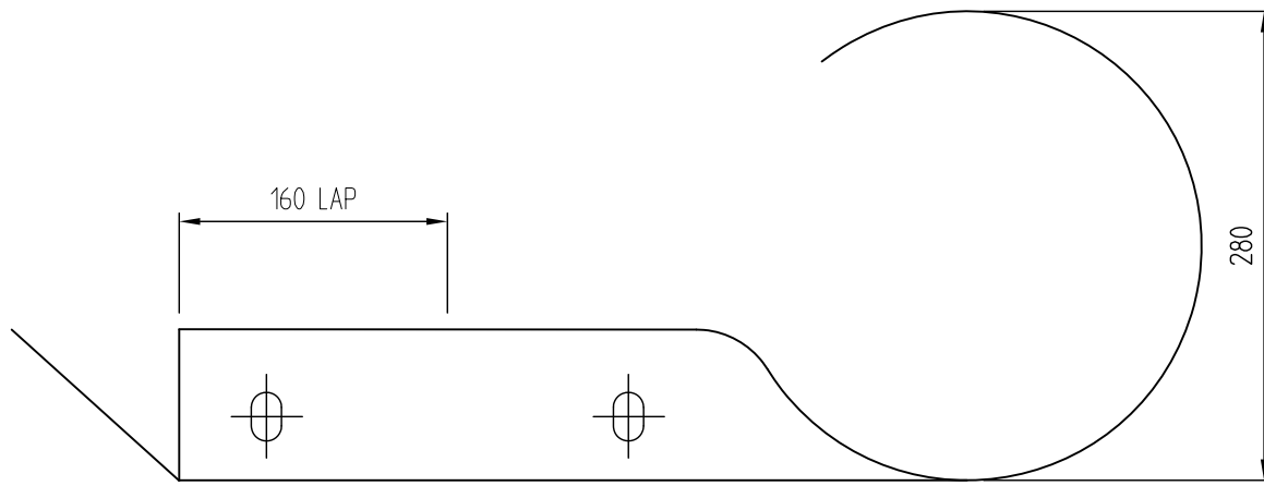
TYPICAL PLAN
