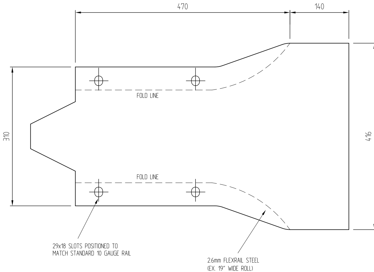
TYPICAL ELEVATION
