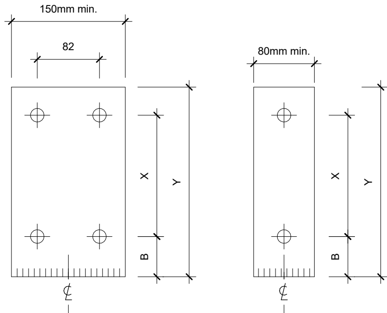
CLEATS AT INTERNAL SUPPORTS (NOT SUPPLIED BY DIMOND)
