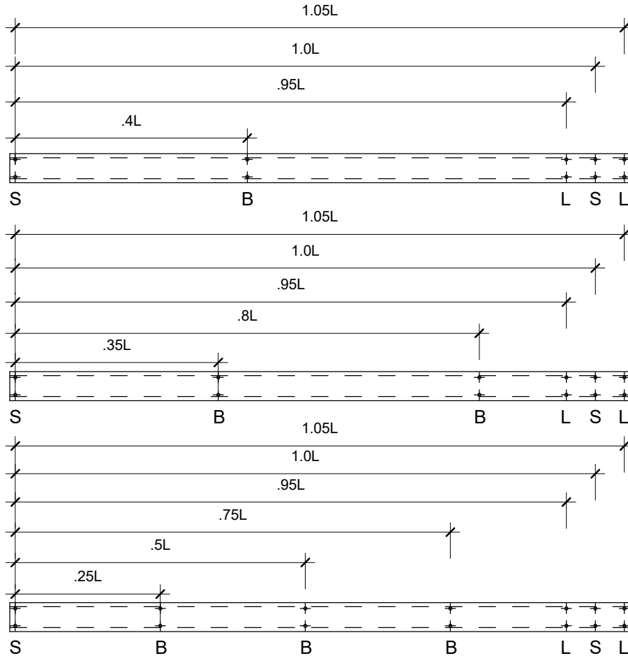
One Brace
