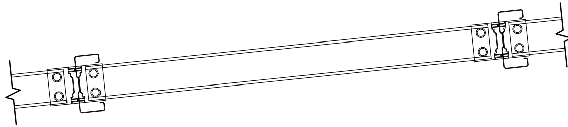
← DHS 150 Bracing Layout - Fastbrace
