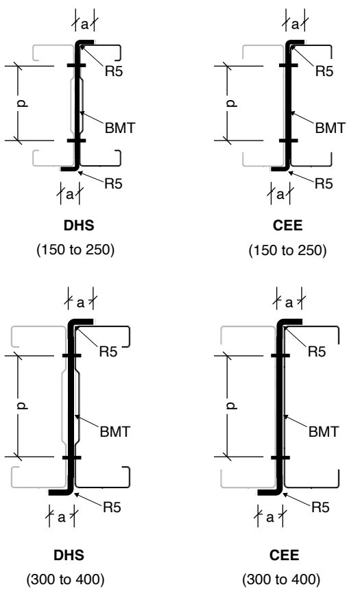
SPLICE PLATE
