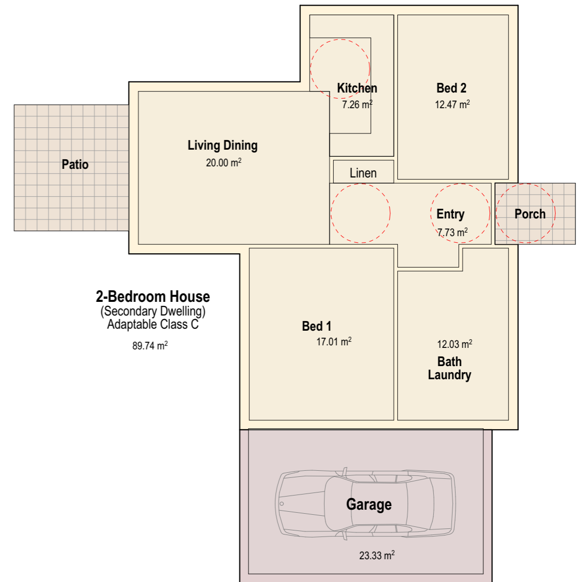
2-Bedroom Secondary Dwelling Plan 1:100
