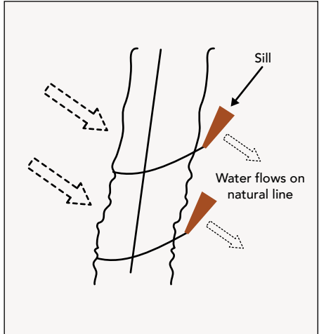
Graded both sides of the fenceline with speed bumps (diversion banks) installed.
