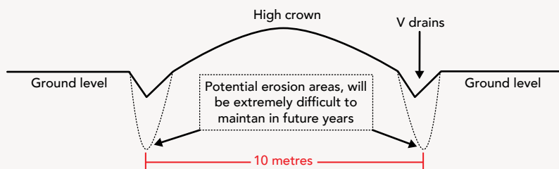
Diagram 1: Road formed too narrow, with no drainage.
