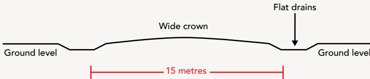
Diagram 1.1: Wide formed road with flat drains.
