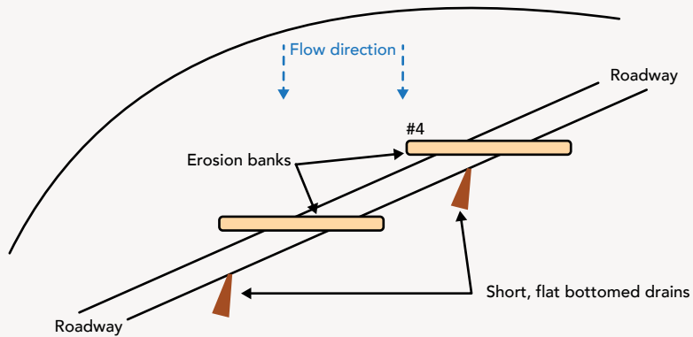
Diagram 3.1: Erosion banks.
