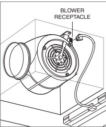
Blower connection
