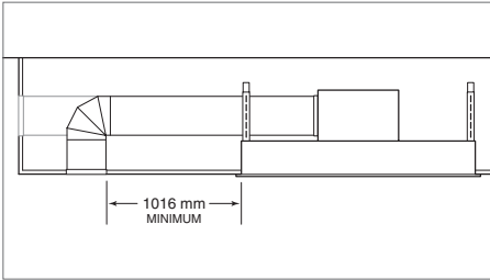
Recirculation application
