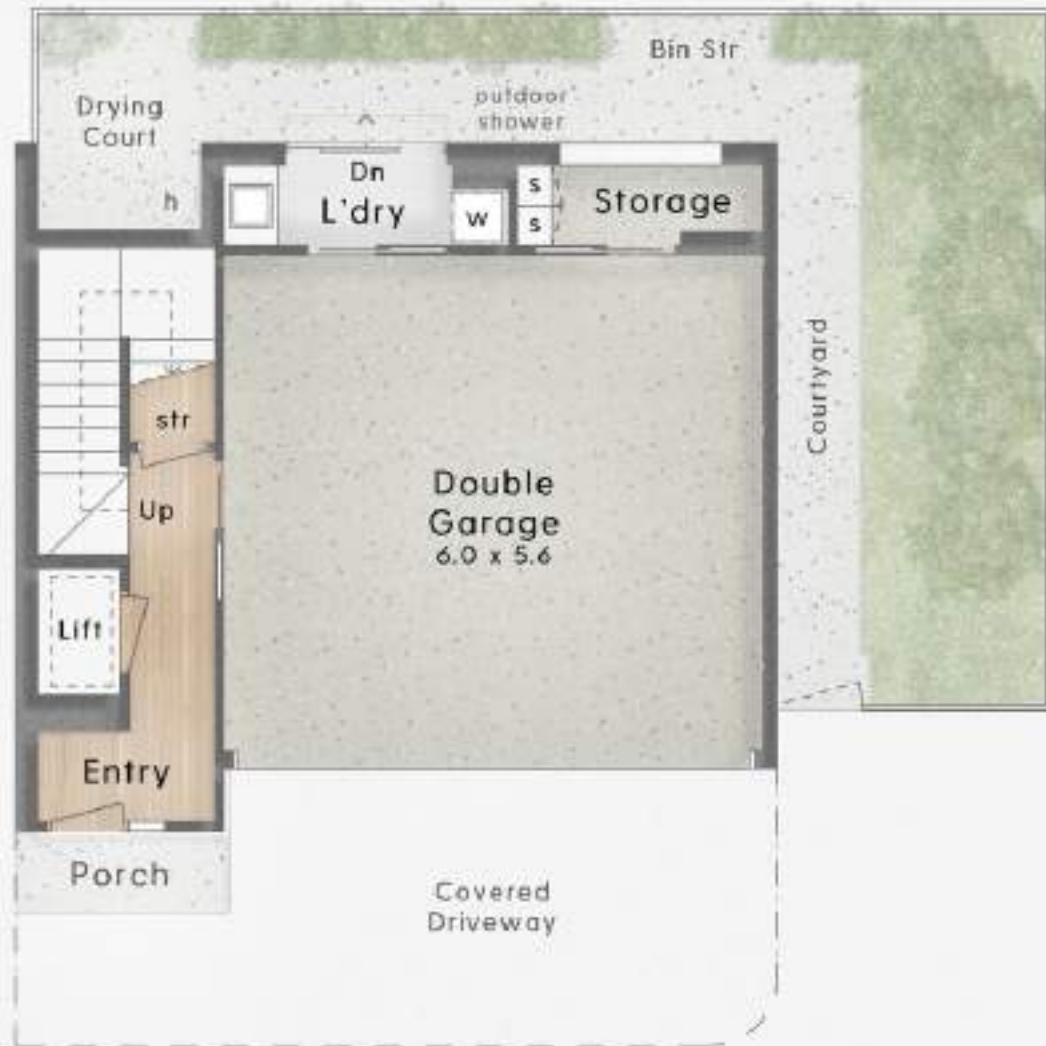
:: FLOOR PLAN Ground Floor
