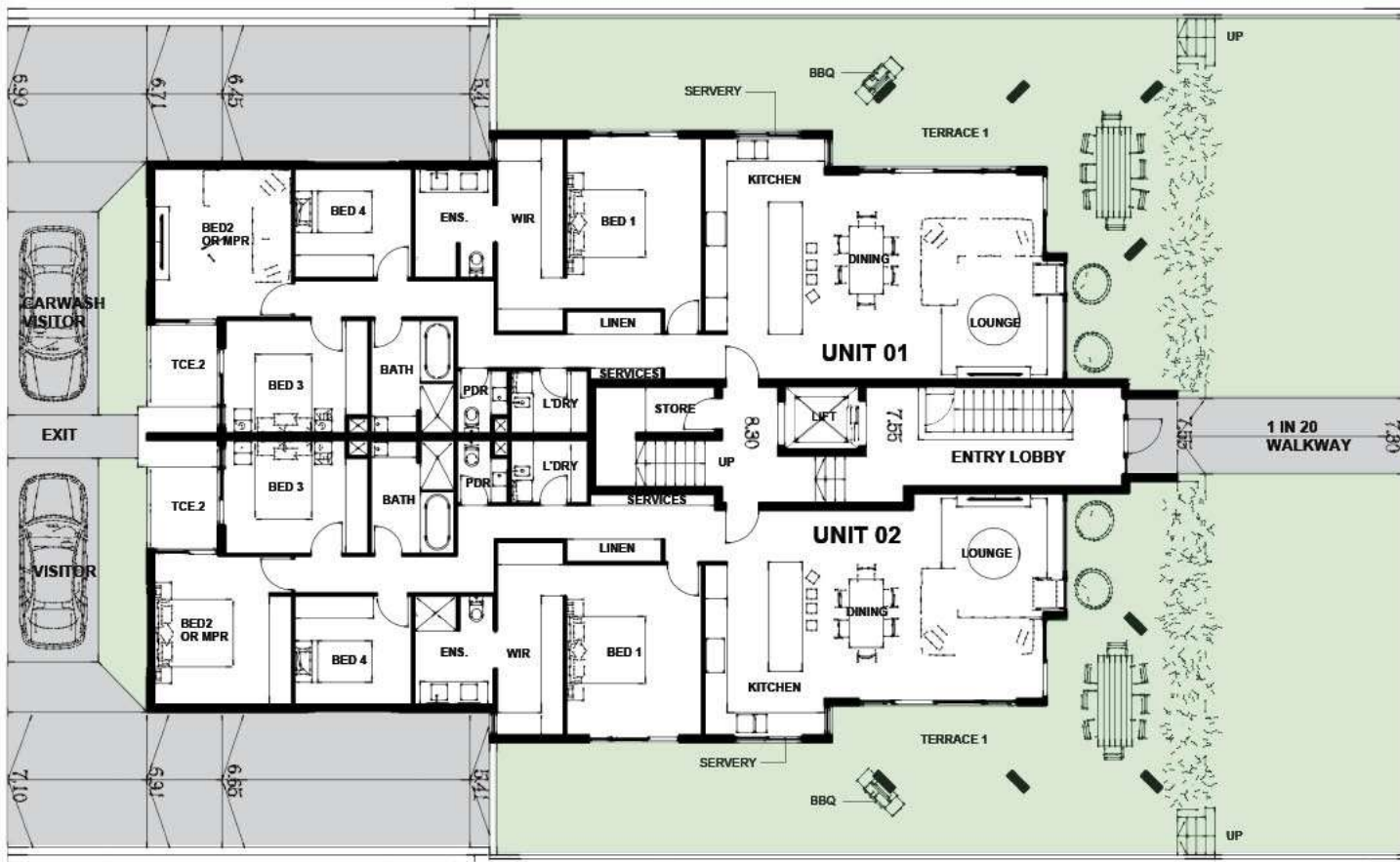
PROPOSED LEVEL 1 FLOOR PLAN
